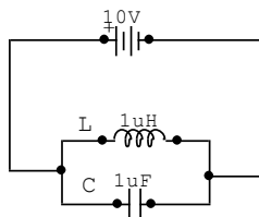
Gambar 12. Rangkaian L-C (CircuitMaker 2000 Software)
