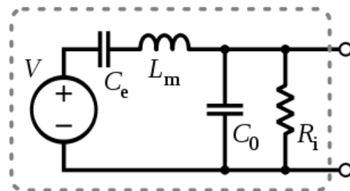
Gambar 2. Piezoelectric Transducer
