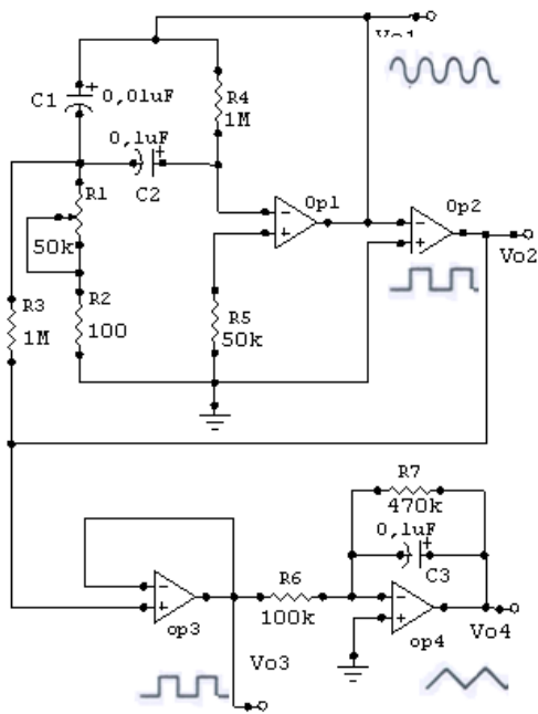
Gambar 19. Osilator Fungsi
