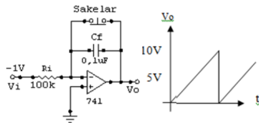
Gambar 19. Osilator Gigi Gergaji
