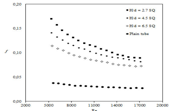
Figure 8. f to Re correlation graph
