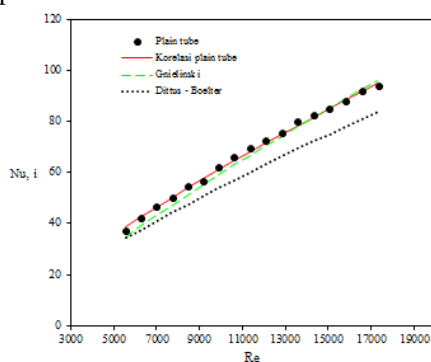
Figure 4. Nu_i to Re correlation on a plain tube graph
