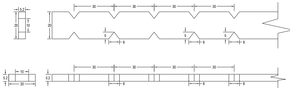
Gambar 5. Benda Uji Bambu Ori Bertakik Jarak 3 cm.
