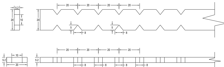
Gambar 4. Benda Uji Bambu Ori Bertakik Jarak 2 cm.
