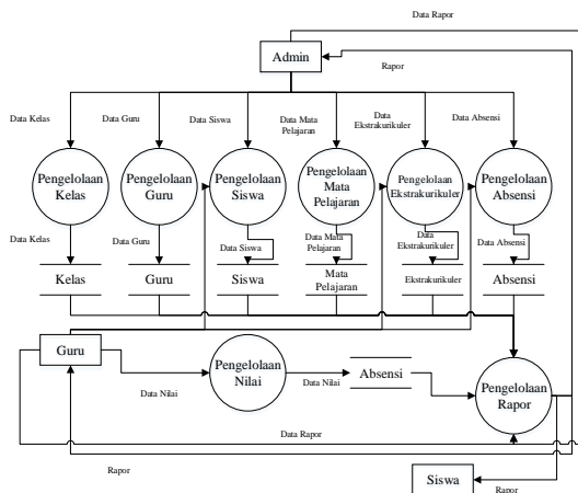
Gambar 8. DFD Level 1
