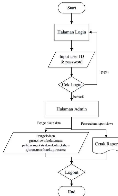
Gambar 6. Flowchart admin
