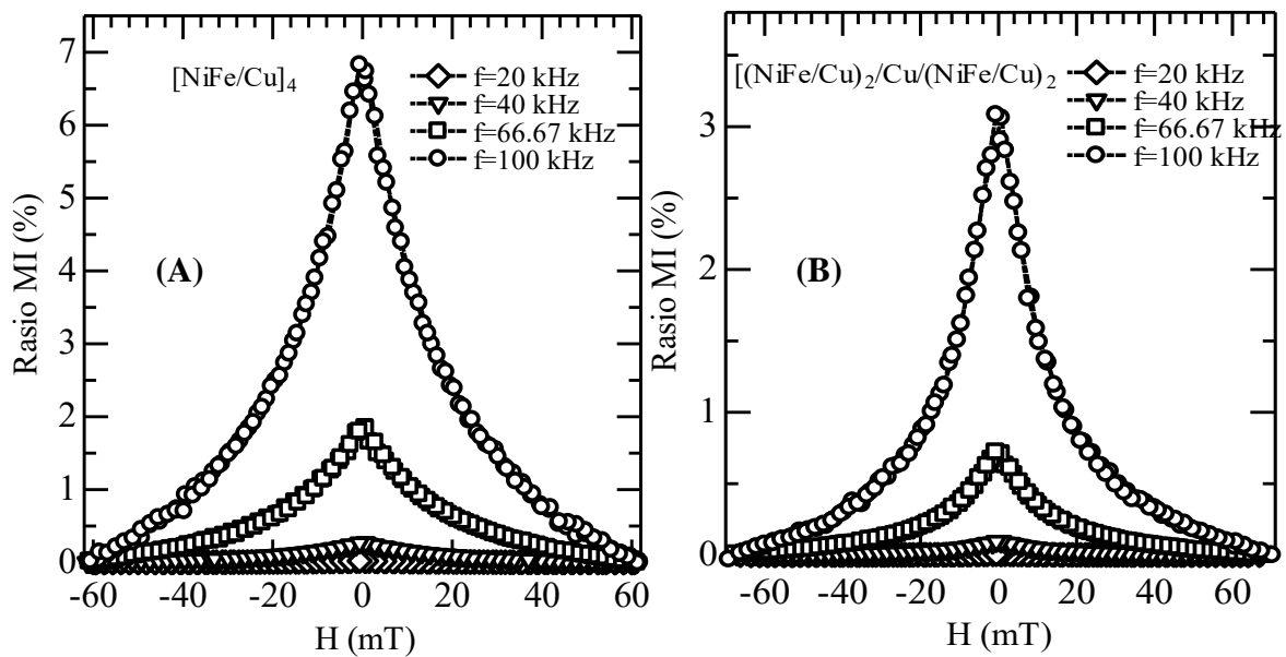
Figure 3. The magnetoimpedance of MI– H curve for sample A of multilayered [\text{NiFe/Cu}]_4 and sample B of multilayered [(\text{NiFe/Cu})_2/\text{Cu}/(\text{NiFe/Cu})_2]
