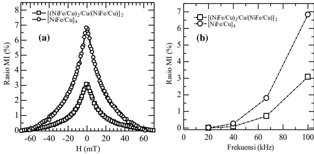
Figure 4. The comparison of the MI ratio in the sample A of the multilayer structure [\text{NiFe/Cu}]_4 and the sample B of [(\text{NiFe/Cu})_2/\text{Cu}/(\text{NiFe/Cu})_2] (a) with a frequency measurement of 100 kHz. (b) The MI ratio versus frequencies of 20, 40, 66.67, 100 kHz
