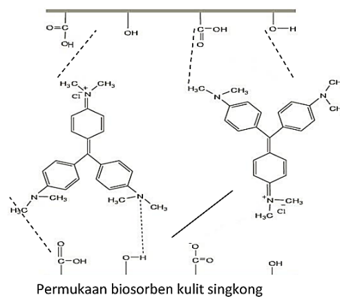
Figure 3. Interaction between crystal violet dye ions with cassava peel adsorbent [21]
