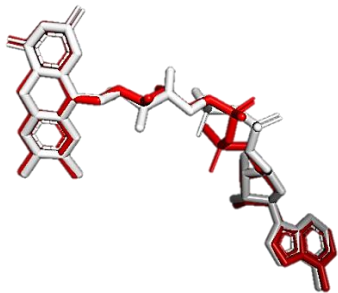
Figure 2. Overlays of redocking ligand (white) with reference ligand from crystallography (red) at 6KGP
