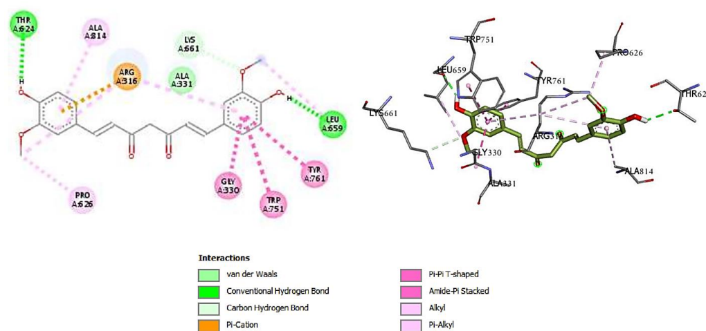
Figure 7. Visualization of docking results 6KGP with 6-shogaol in 2D and 3D
