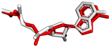
Figure 1. Overlays of redocking ligand (white) with reference ligand from crystallography (red) at 3SWR
