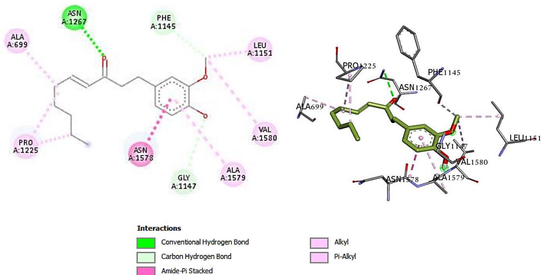
Figure 3. Visualization of validation results 3SWR with sinefungin in 2D and 3D
