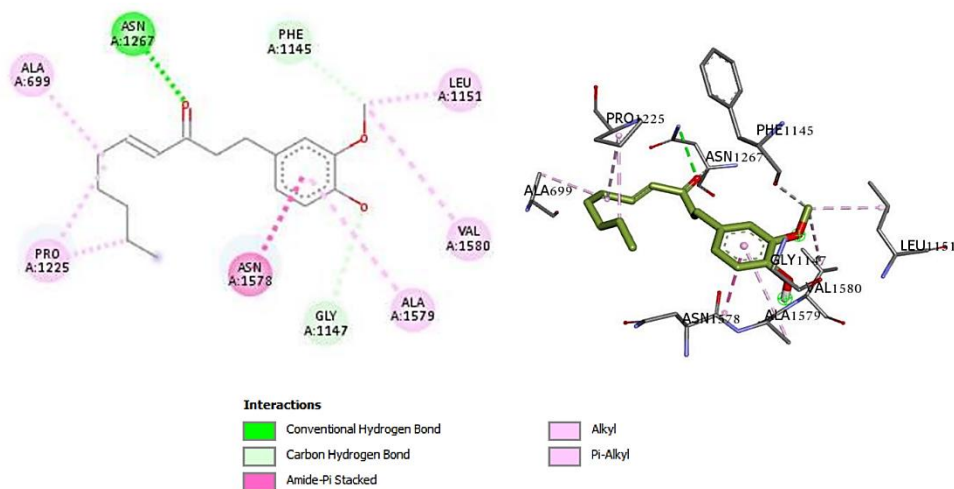
Figure 6. Visualization of docking results 3SWR with 6-shogaol in 2D and 3D
