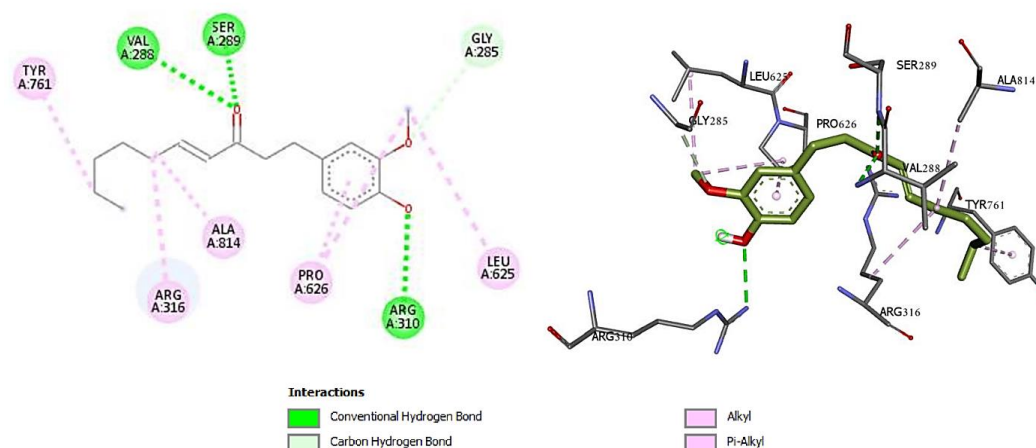
Figure 7. Visualization of docking results 6KGP with 6-shogaol in 2D and 3D
