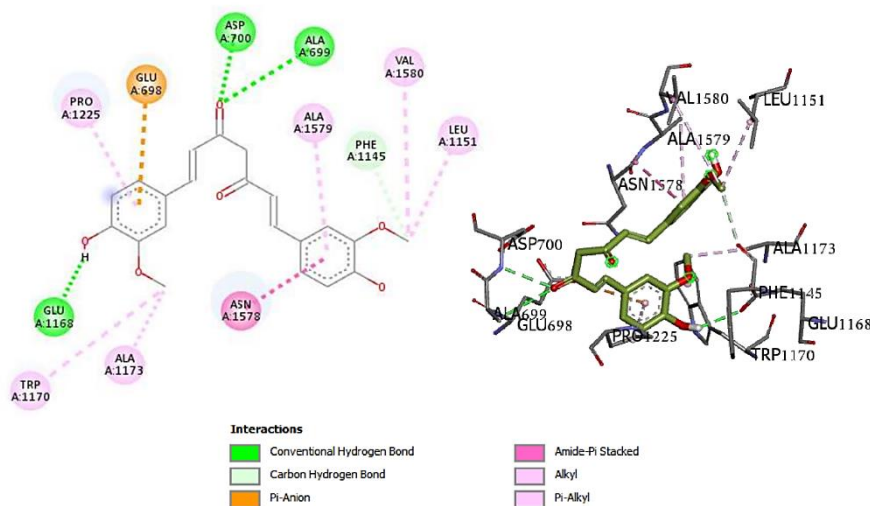
Figure 5. Visualization of docking results 3SWR with curcumin in 2D and 3D
