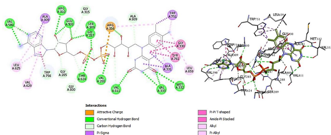
Figure 4. Visualization of validation results 6KGP with FAD in 2D and 3D
