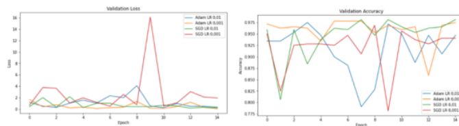
Figure 5. Evaluation Model
