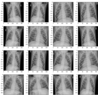
Figure 4. Augmentation Data
