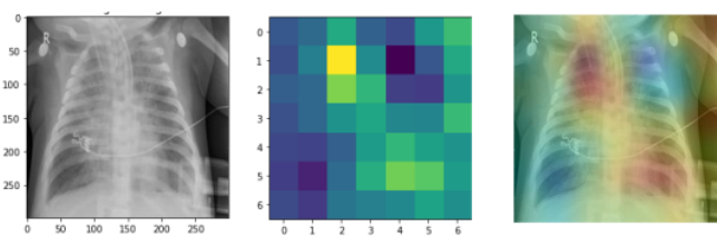
Figure 6. Grad-CAM
