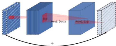
Figure 2. MBConv Block
