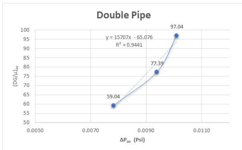
Figure 3.2. Relationship Graph (DG/\mu)_{av} vs \Delta P_{av} in Double Pipe
