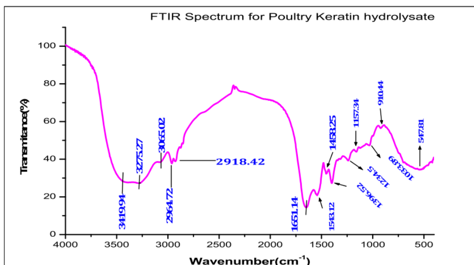
Figure S1. The FTIR Spectrum for Reference Keratin (Mengistu et al., 2024)
