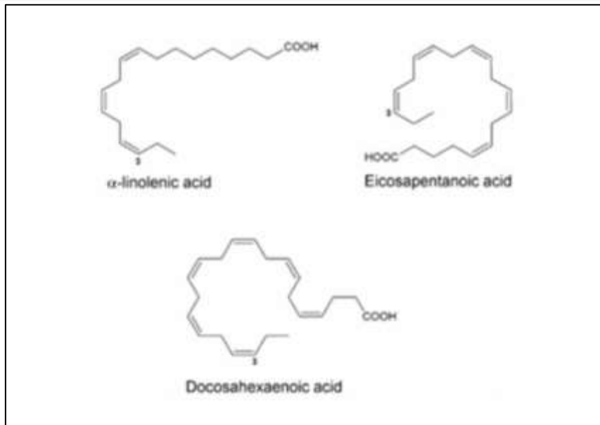
Figure 1. Chemical structures of the three primary omega-3 fatty acids: \alpha -linolenic acid (ALA, C18:3n-3), eicosapentaenoic acid (EPA, C20:5n-3), and docosahexaenoic acid (DHA, C22:6n-3)
