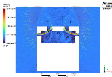
Figure 11. Air Flow Velocity in the Hawu
