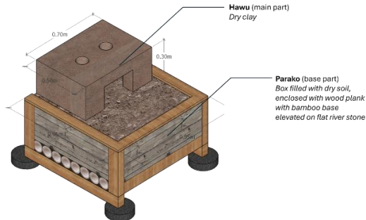
Figure 2. Dimension of Hawu
